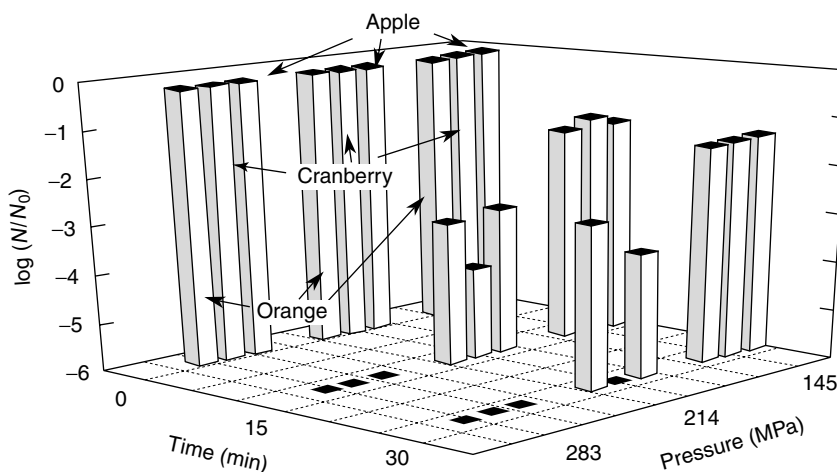
FIGURE 34.19 Effect of high-pressure treatments on Saccharomyces cerevisiae inoculated in apple, cranberry, and orange juices. (Adapted from D. G. Hoover et al., Food Technol. 43(3):99, 1989.)
