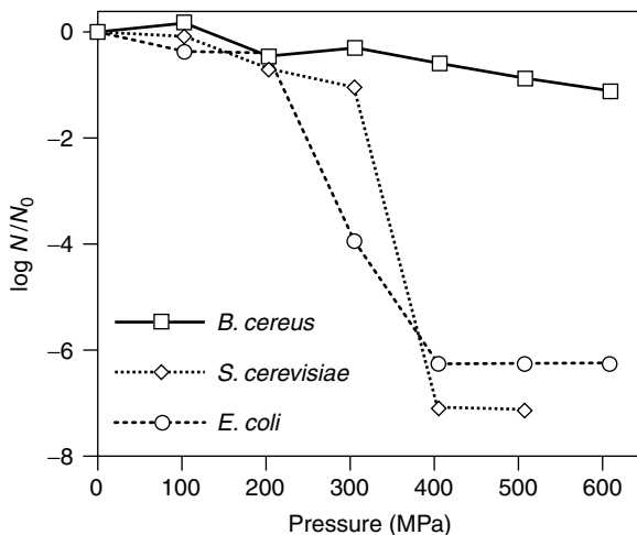
FIGURE 34.5 Effects of high hydrostatic pressure on Bacillus cereus spores and Saccharomyces cerevisiae and Escherichia coli vegetative cells inoculated into pork slurries. The inoculated samples were subjected to pressure treatments for 10 min at 25°C. N and N_0 represent the number of survivors and initially inoculated microorganisms, respectively. (Adapted from T. Shigehisa et al., Int. J. Food Microbiol. 12:207, 1991.)
