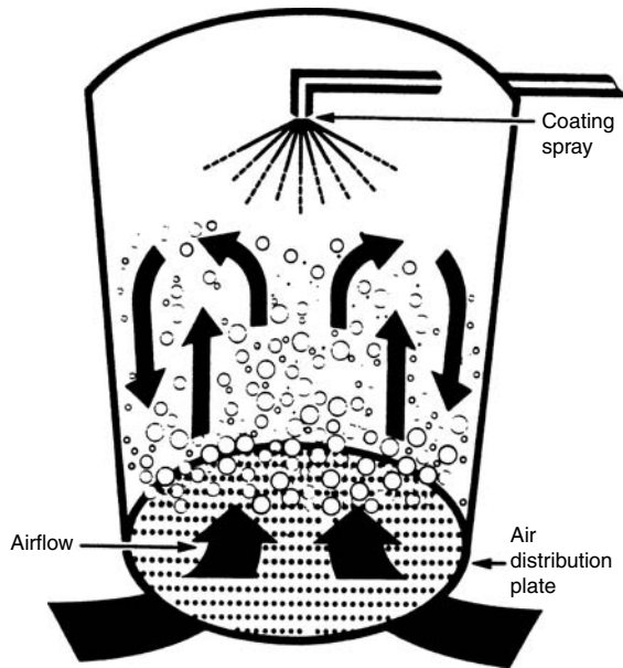
FIGURE 22.8 Schematic representation of a conventional air suspension system. (From J. D. Dziezak, Food Technol. 42(4): 136, 1988.)
