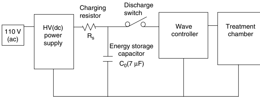
FIGURE 33.3 Major components of commercial electroporator GeneZapper.
