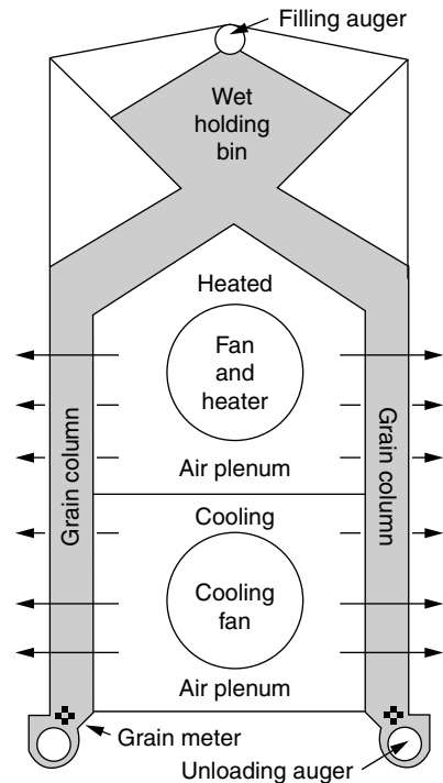
FIGURE 4.26 Cross-flow dryer with forced-air drying and cooling. (From K.J. Hellevang, W.F. Wilcke. Maintaining corn quality for wet milling . AE-1119, Extension Service, North Dakota State University, Fargo, ND, 1996.)
