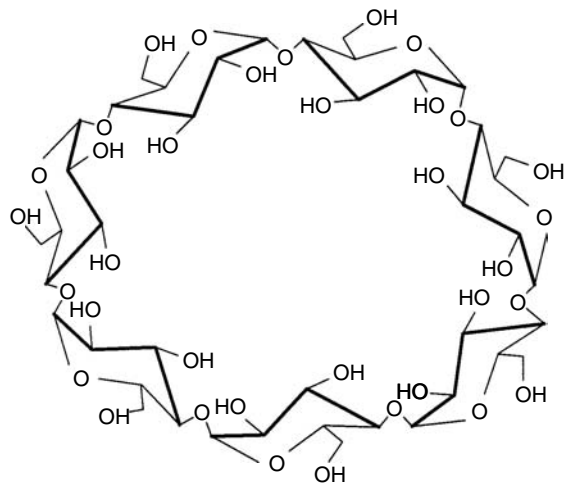
FIGURE 22.3 Chemical structure of \beta -cyclodextrin.
