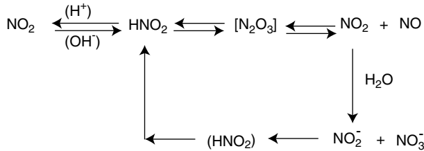
FIGURE 13.1 The dynamics of nitrous acid production in a cyclic reaction. (Adapted from Shank et al., Appl. Microbiol. 10:185, 1962.)
