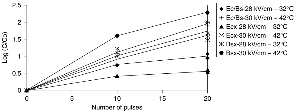
FIGURE 33.22 Inactivation of mixture of microorganisms suspended in pea soup using PEF at 0.75 L/min and 4.3 Hz (Ec: E. coli ; Bs: B. subtilis ; Ec/Bs: the overall inactivation for the mixture of microorganisms; Ecx: the inactivation of E. coli in the mixture; Bsx: the inactivation of B. subtilis in the mixture). (From H. Vega-Mercado et al., J. Food Proc. Pres. 20(6): 501, 1996.)
